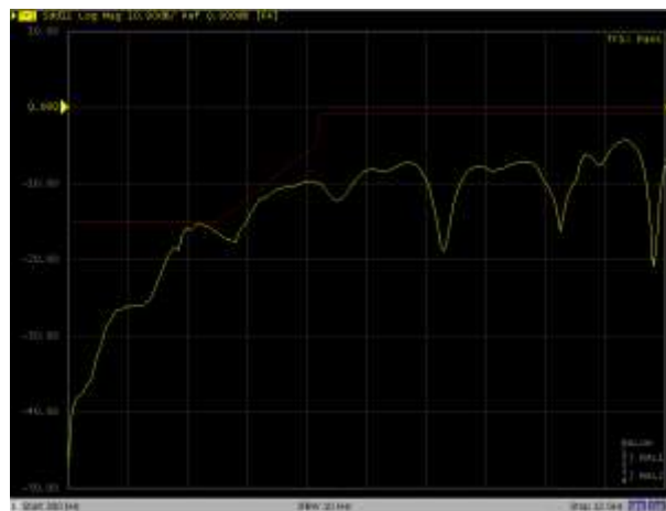
Return Loss
