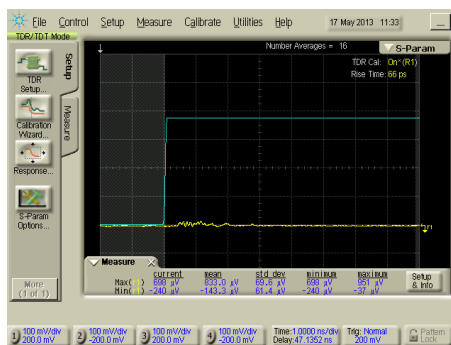
Crosstalk
