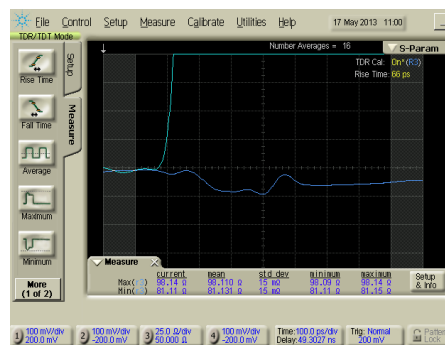
Impedance
